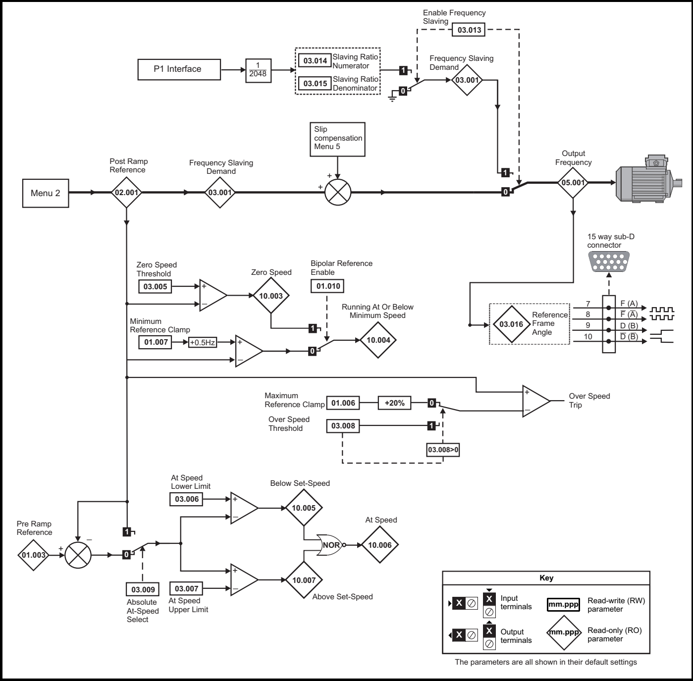
Figure 11-3 Menu 3 Open-loop logic diagram
